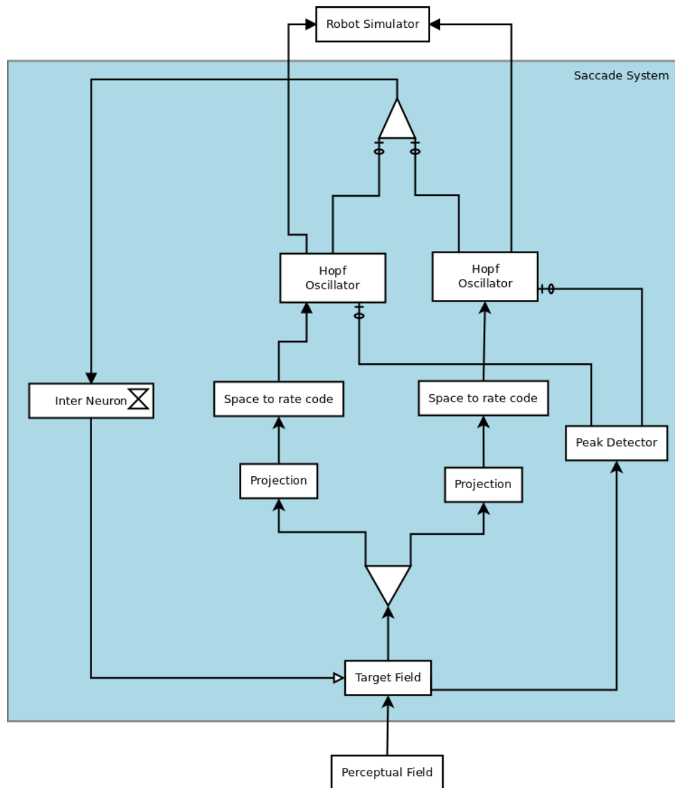
Figure 4.5: Sequence of the saccade system
