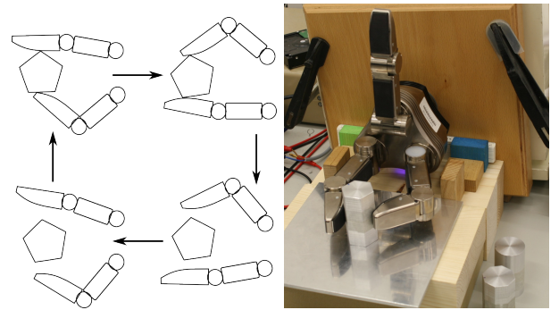
Fig. 3. Left: sketch of the rotation behaviour; Right: picture of our experimental setup
