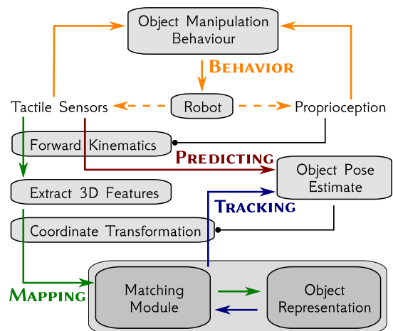
Fig. 1. Overview of the general architecture: black lines with a dot at the end indicate a parametrization relationship. Arrows pointing to boxes indicate inputs for processing in the box, and arrows passing through boxes indicate a parametrized transformation of the information through the box.
